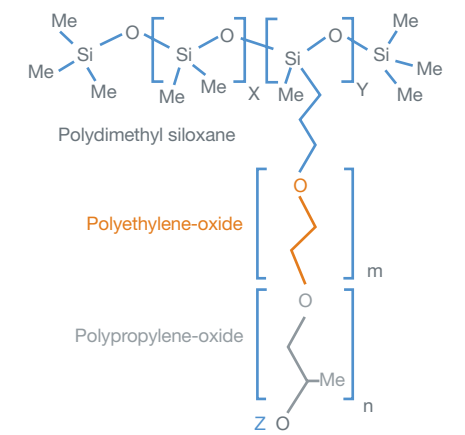
Silicone-polyether block copolymer-pendant structure
