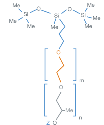
Trisiloxane structure
